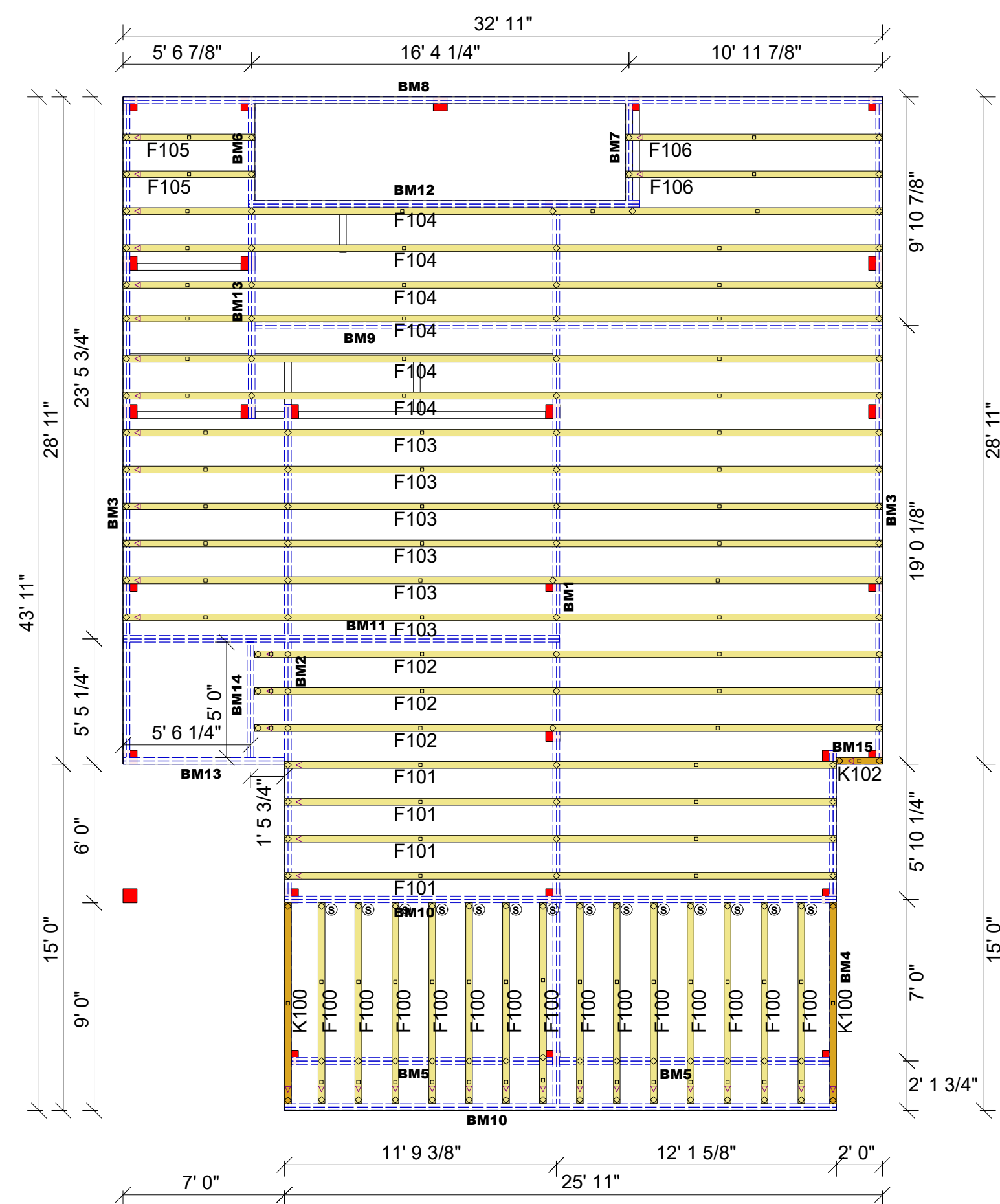
FIRST FLOOR PLACEMENT PLAN
