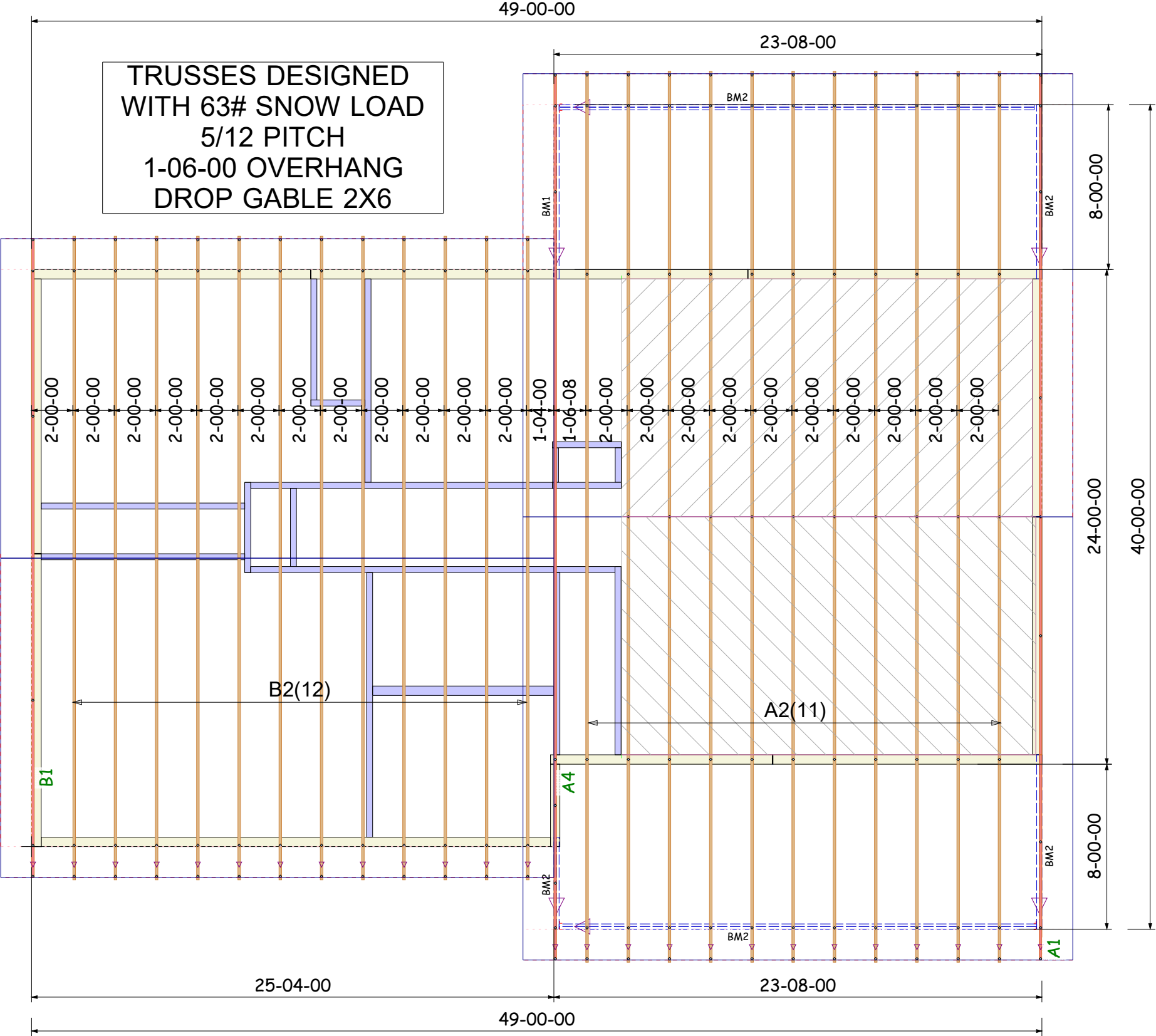
Roof Layout
