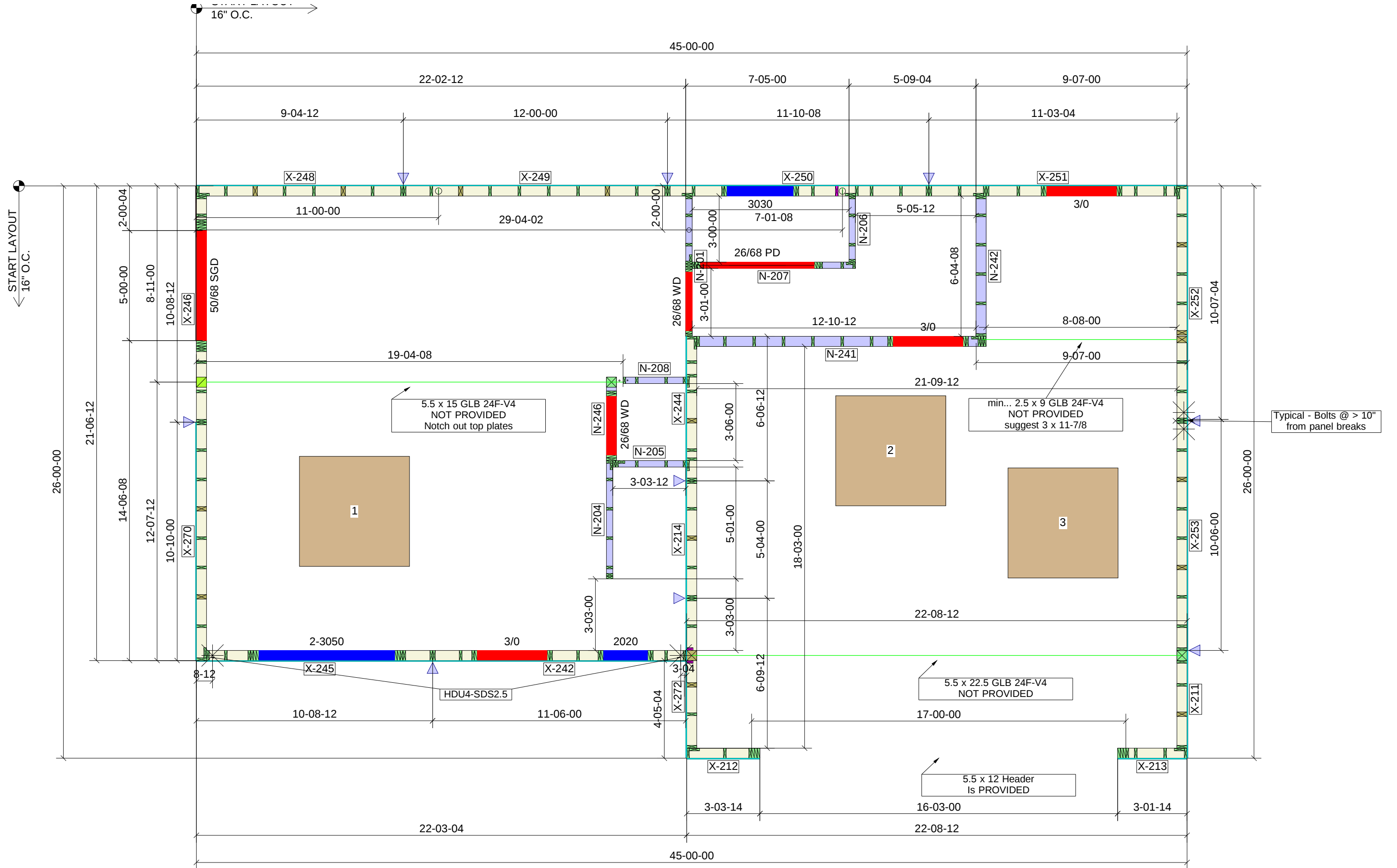
First Floor
