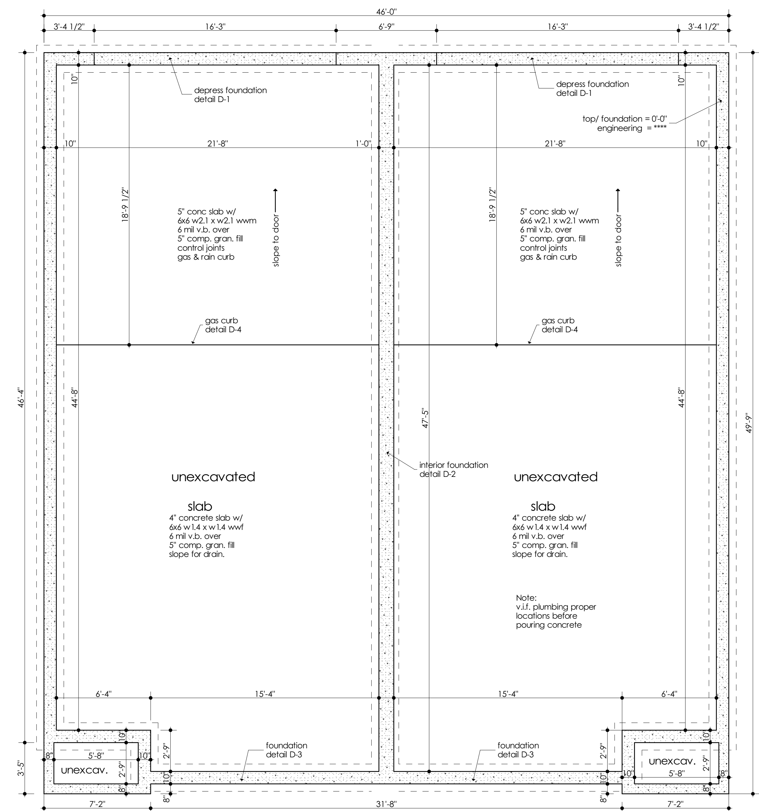
Foundation plan
