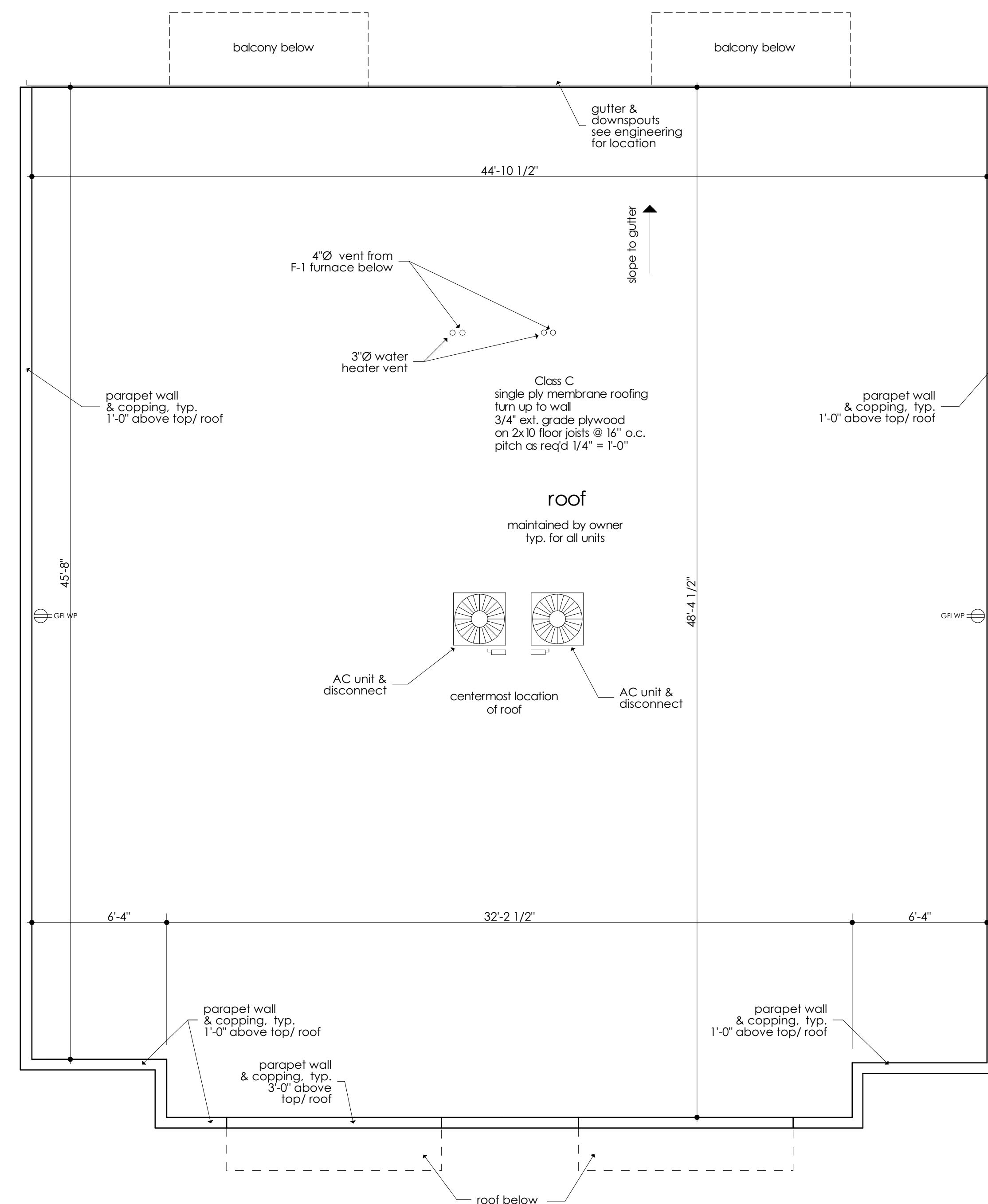
Roof plan
