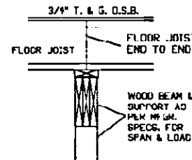
CENTER BEARING SUPPORT OPTION S-2
